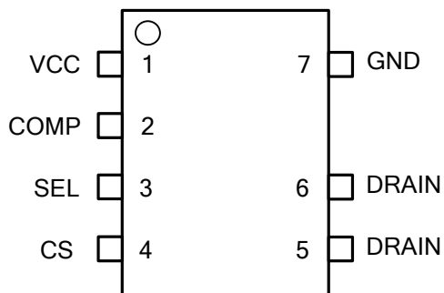
SOP-7/DIP-7
